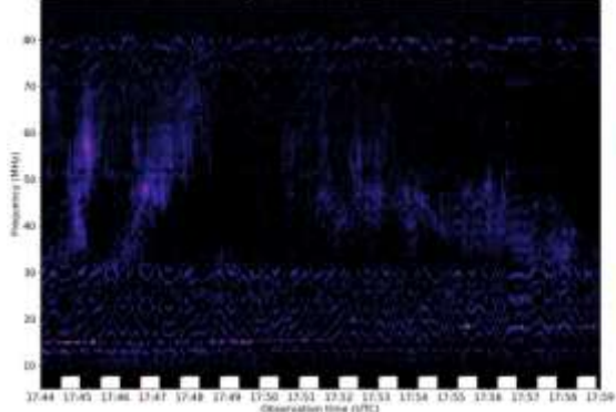
2026/05/16 Radio flux density, e-CALLISTO (ALASKA-COHOE), Focuscode = 63
