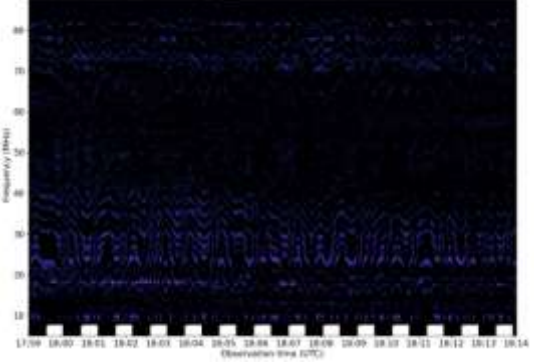
2026/05/16 Radio flux density, e-CALLISTO (ALASKA-COHOE), Focuscode = 62
