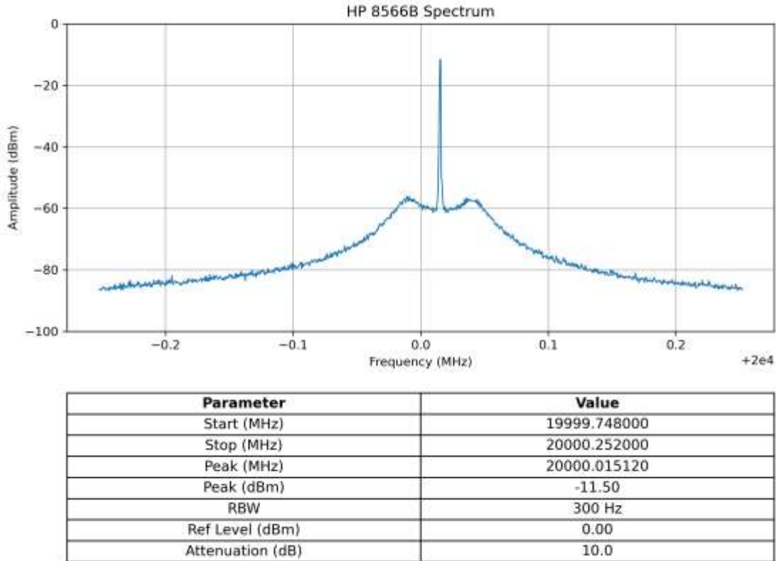
Fig. 5: Phase noise at 20 GHz
