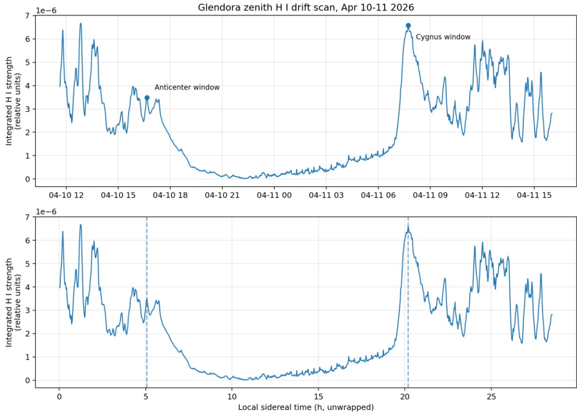
Figure 5: Integrated H I strength versus time and sidereal time for the 10–11 April 2026 case-study run.
