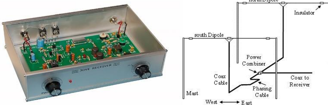
Figure 1. A Radio JOVE RJ1.1 receiver and a schematic of the dual-dipole antenna.
