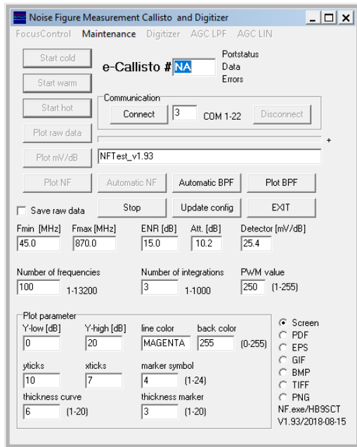
Figure 1 ~ Main window when NF Test is first opened and not yet Connected to the instrument through the serial port. At this point, the Connect button may be pressed if the Communication COM port is correct; otherwise, before pressing Connect, it is necessary to change the COM port to match the serial port to be used.
