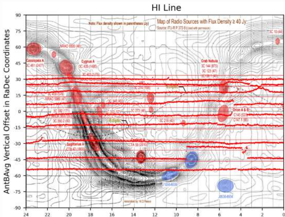
Figure 5 - Right Ascension - Declination Map of the Galaxy
