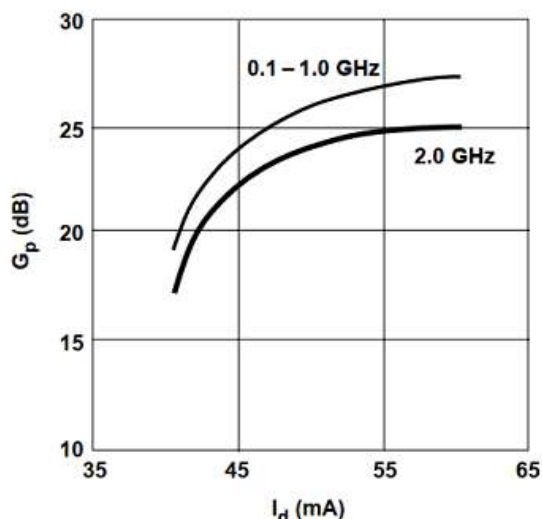
Figure 3. Power Gain vs. Current.
