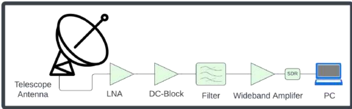
Figure 2 - Block Diagram of the Components for the Telescope Receiver Chain
