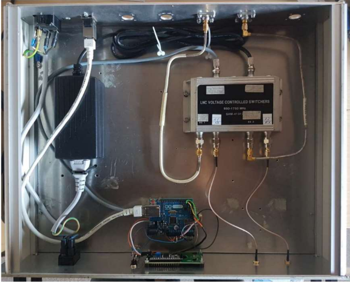
Figure 3: Control unit for LNB
