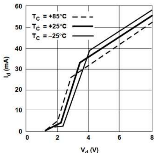
Figure 2. Device Current vs. Voltage.
