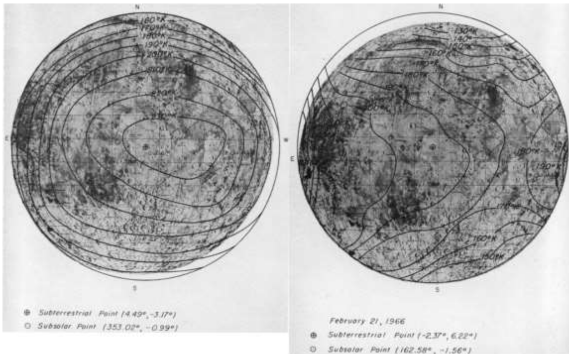
Figure 1: The observed distributions of radiation temperatures across the lunar disk [2]. At left – wavelength 8.6 mm, phase 12° after Full Moon, at right – wavelength 3.2 mm, phase 196° after Full Moon (or 16° after New Moon).
