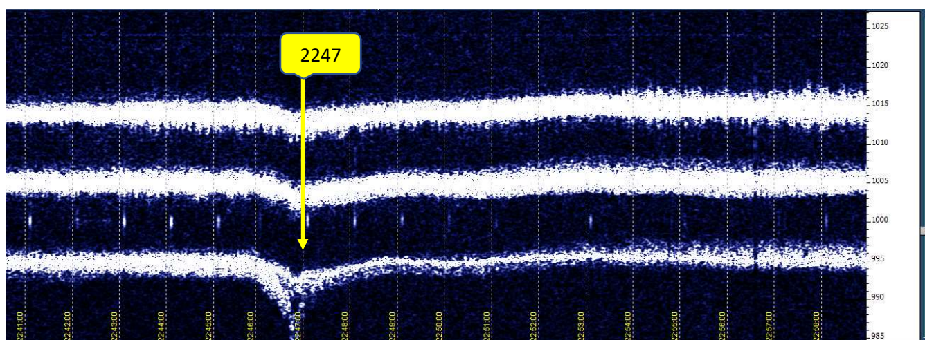
Figure 1 ~ Argo plot for 2241 to 2259 on 10 January 2023 UTC showing an SFD starting at 2246. The yellow time hack is placed near the SFD peak of about -10 Hz frequency deviation at 15 MHz. The SFD is most pronounced at 15 MHz and almost nonexistent at 25 MHz. The propagating carrier encountered additional absorption for several minutes afterwards at 15 MHz by the added ionization in the ionosphere's D-region. The SFD was caused by an impulsive X1.0 flare at solar Active Region 3186 beginning at 2239, peaking at 2247 and ending at 2252.
