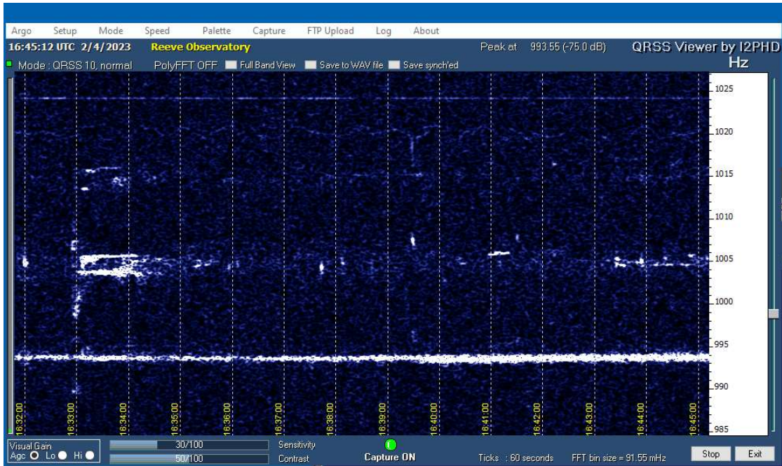
Figure 2 ~ Argos plot for 1632 to 1645 on 4 February 2023 UTC showing a long duration echo at 20 MHz (middle trace at 1005 Hz) and the vestige of an echo at the same time on 25 MHz (upper trace at 1015 Hz). A number of short duration echoes are seen at 20 MHz. The 15 MHz carrier (lower trace at 995 Hz) is continuous but very weak and shows no echoes.
