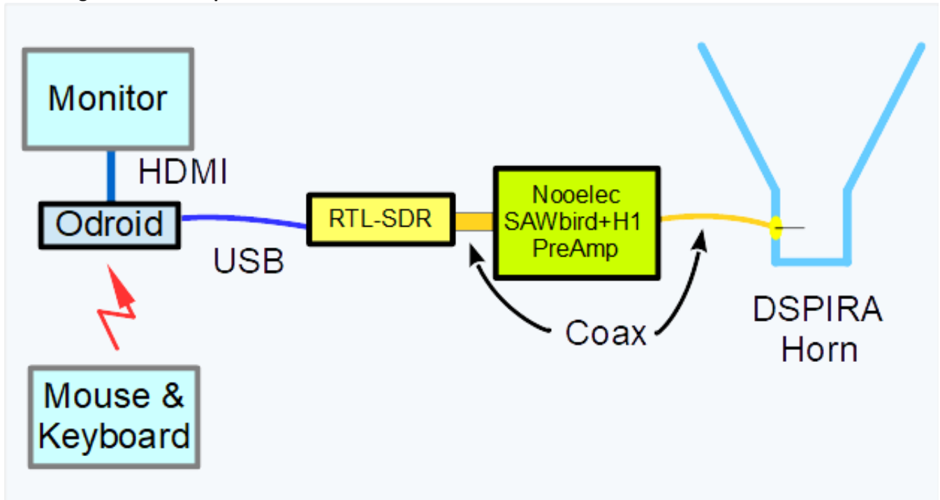
Setup Diagram
