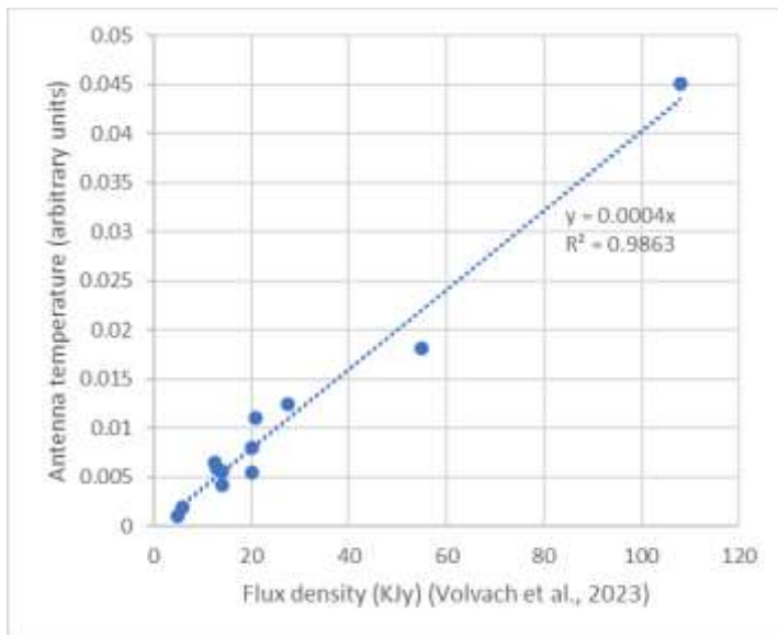
Figure 3: correlation between measurements of the 1 metre dish and reported flux density of the flare.
