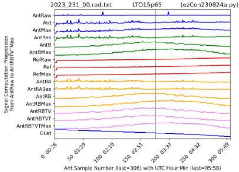
A condensed graph of different kinds of processing. The black vertical line in the middle indicates where the antenna crosses the galaxy, in which from the more filtered versions (pink) it could be seen that intensity detected is higher near the galaxy.
