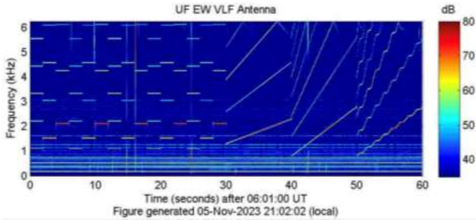
Figure 4 ~ HAARP induced ULF and VLF emissions received at Chistochina about 30 km northeast of HAARP on 5 November from a similar experiment. Acknowledgements: Robert Moore – University of Florida for ELF Receiver & Mark Golkowski – University of Colorado for the experiment sequence
