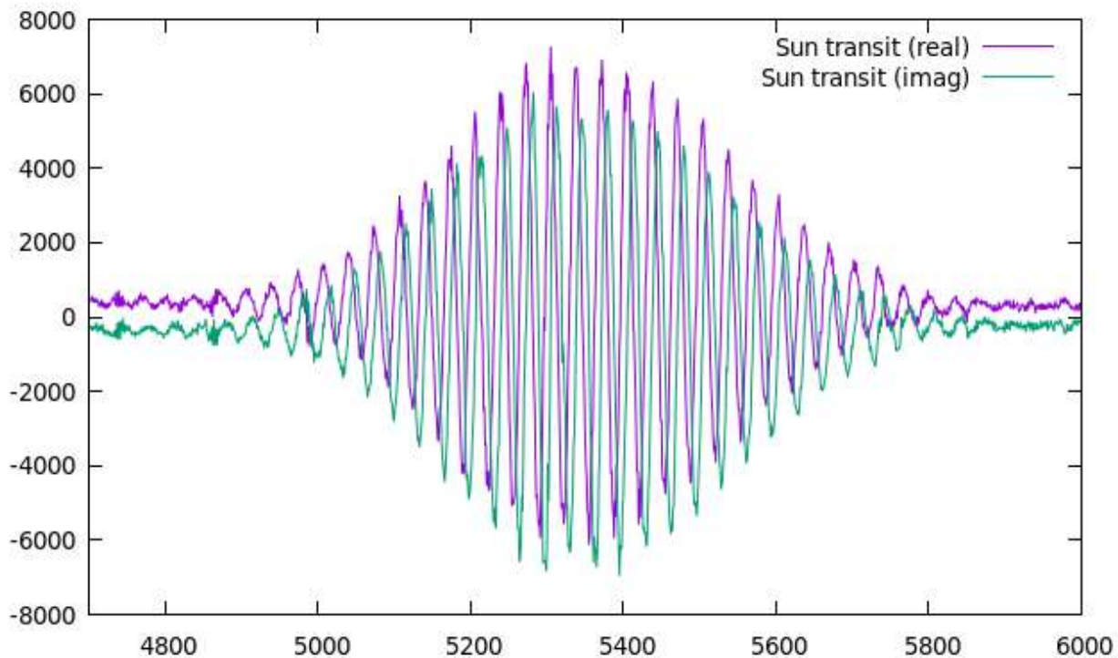
Figure 6: Fringes from a sun transit
