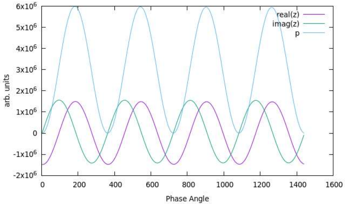
Figure 3: Recorded phase and power signal
