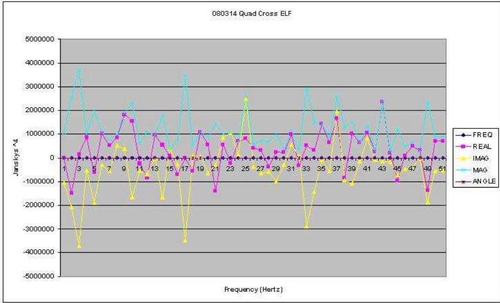
Illustration 8: This is the result of a Quad Cross Correlation starting at 0 Hertz to 100 Hertz (in 2 second bins). When Angle, Real, Imaginary, and Magnitude values (Jansky measures) are positive there may be a significant correlation between the two frequencies and a possible indication of a mixture of polarizations at different amplitudes, and altitudes on the sun.
