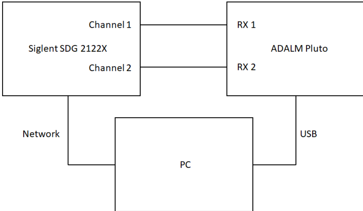
Figure 2: Test Setup
