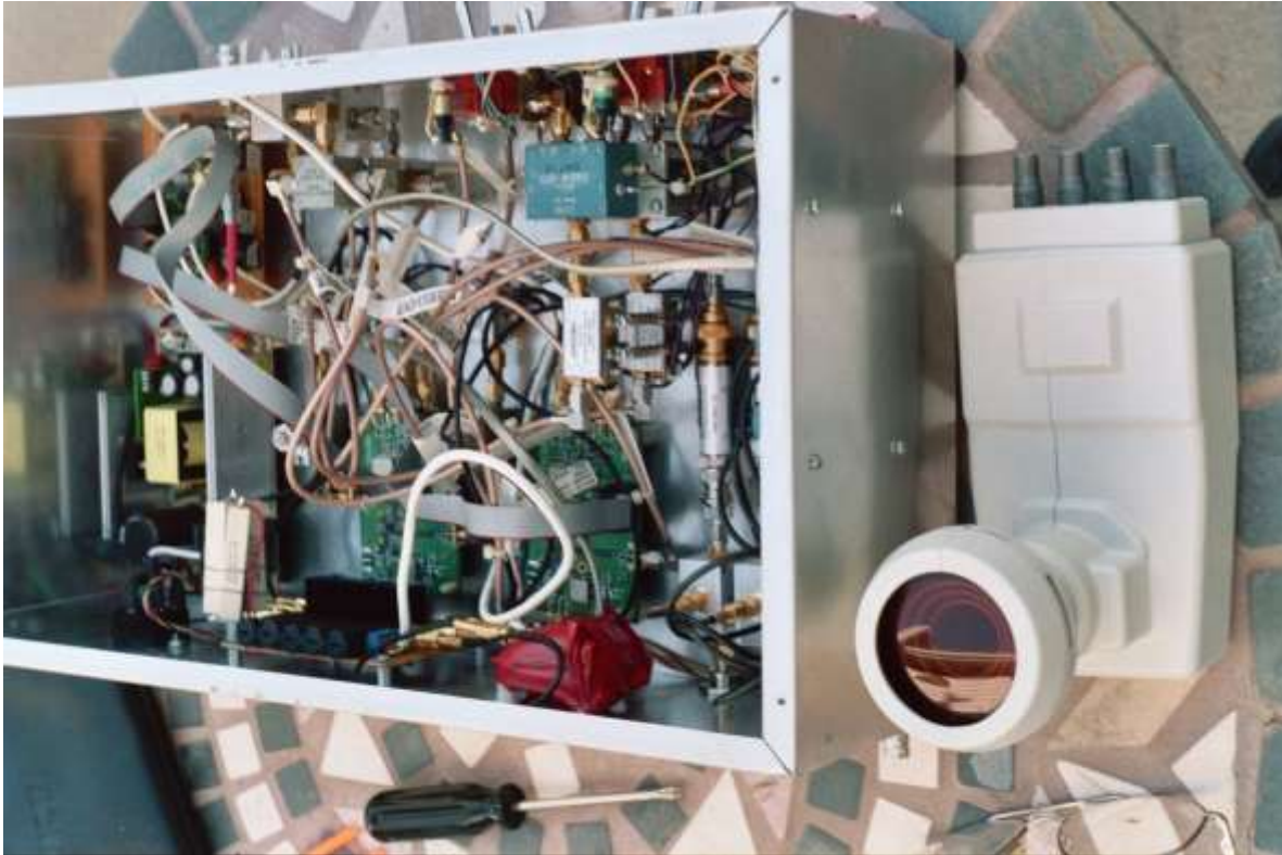
Illustration 2: Paul Oxley's receiver (left), Invacom QPH-031 dual polarity dual frequency LNB (right).
