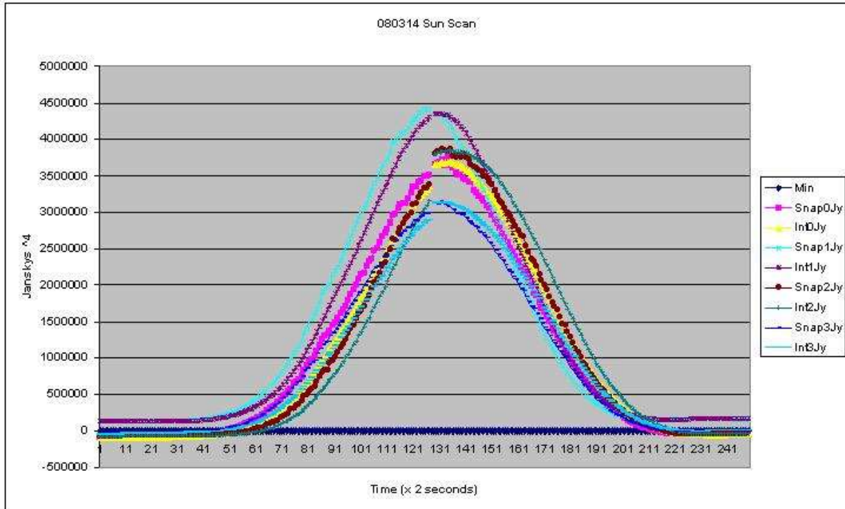
Illustration 6: Channels 0 - 3 during a Sun Scan. There is pause near the peak where a 2 minute snapshot of data was taken for the Quad Cross Correlation routines to examine the polarization of Vertical, Horizontal, Right Circular and Left Circular polarization measured in Janskys.
