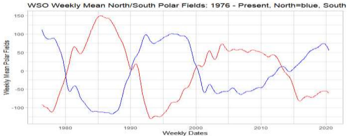
Figure 2 shows the WSO solar magnetic cycles from 1976 to 2020.
