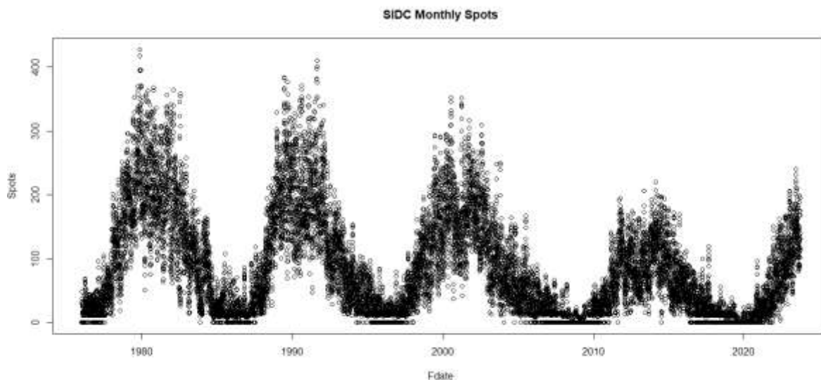
Figure 1 shows the SSN cycle from 1976 to 2023
