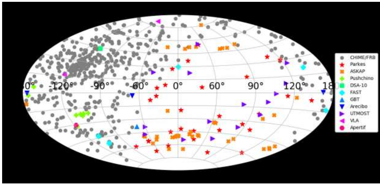
Figure 1: Currently known sample of FRBs in galactic coordinates (E. Petroff, et.al, arXiv:2107.10113v2 [astro-ph.HE] 19 Jan 2022)
