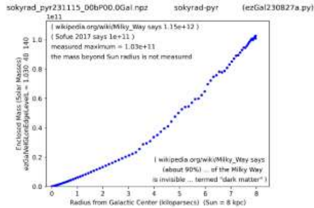
Figure 8: Calculated Galactic Mass
