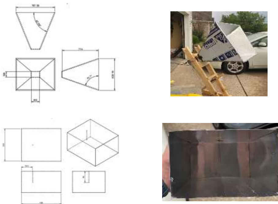
Figure 1: Dimensions and Photos of Antenna
