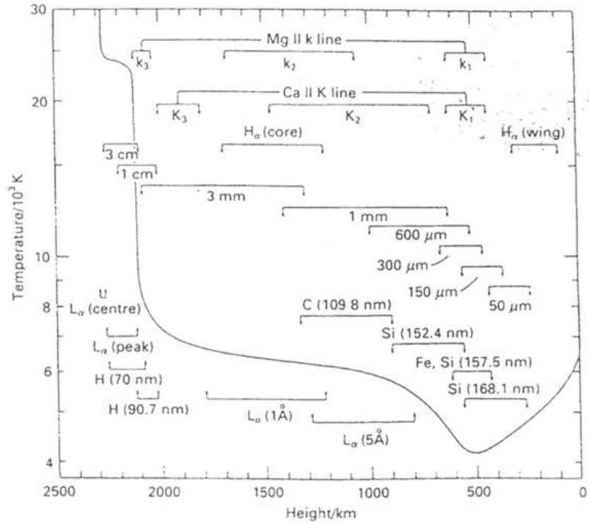
Illustration 9: The altitudes of the transition region for the temperature region being recorded, i.e., between 11.7 GHz and 12.2 GHz, above the photosphere. As there may be differences in polarizations of the transition region during active flares on the sun, these are only estimates as in this Athay Chart, (1986).
