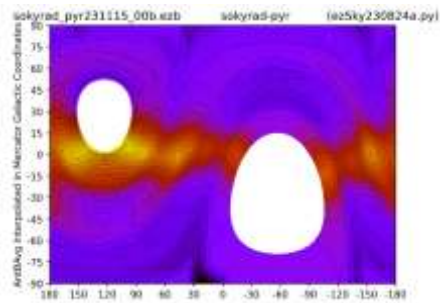
Figure 3: Mercator Plot
