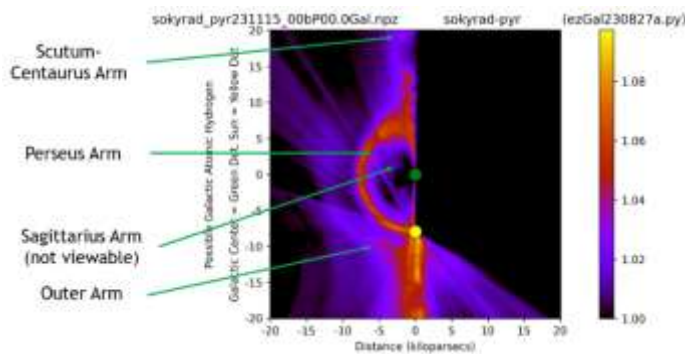
Figure 4: Distance from Galactic Center
