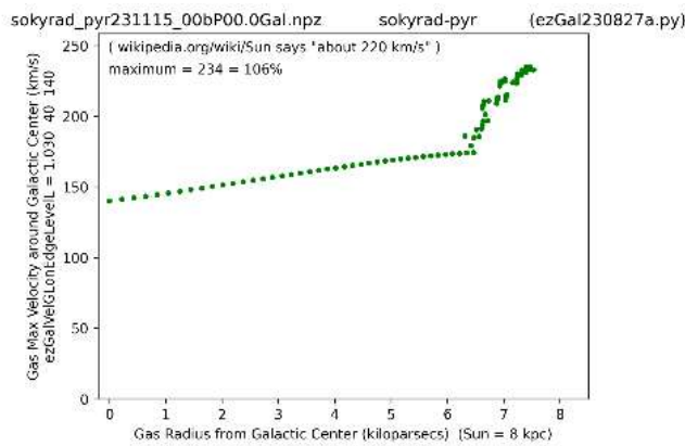
Figure 7: Calculated Gas Velocity
