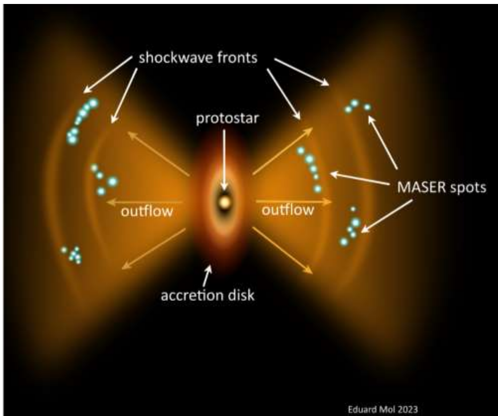
Figure 4: conceptual model of masers around a protostar.
