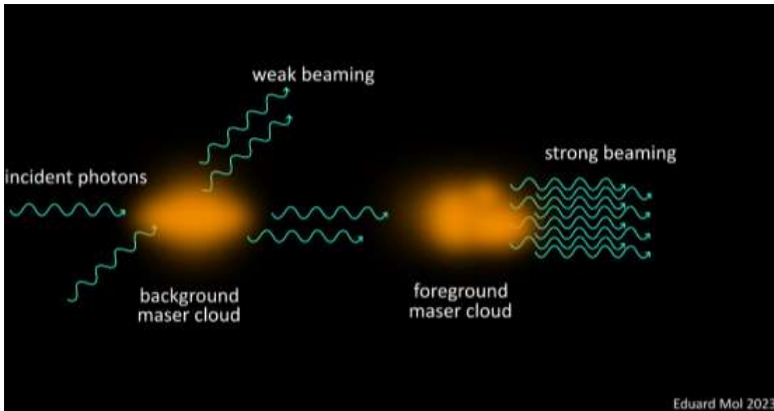
Figure 5: illustration of maser beaming due to maser clouds overlapping along the line of sight. Note that the foreground cloud can only amplify the radiation from the background cloud if both clouds are moving at the same velocity along the line of sight. If the foreground cloud is moving at a different velocity with respect to the background cloud, the radiation from the background cloud is slightly red- or blueshifted away from the water line frequency and thus cannot be amplified.
