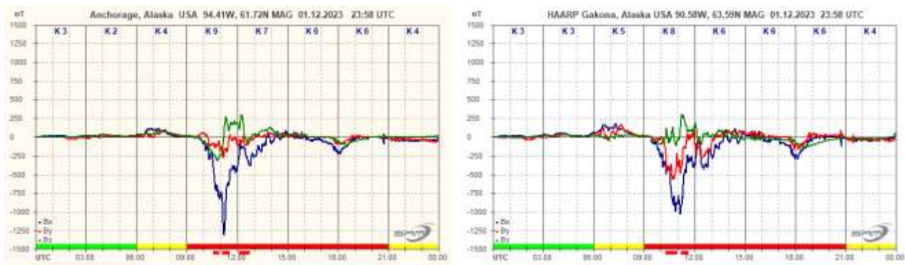
Figure 1 ~ Magnetograms from the SAM-III magnetometers at Anchorage and Gakona, Alaska for the 24-hour period 1 December 2023. The two sites are about 290 km apart and differ in magnetic latitude by about 2° and longitude by about 4°. The CME impact occurred at 0020 UTC and cannot be discerned in the traces because of the high vertical scale. About 6 hours after the sudden impulse, the magnetic field showed a brewing storm and just before 1000 experienced a major disturbance with the K-index going to maximum value (K9).
