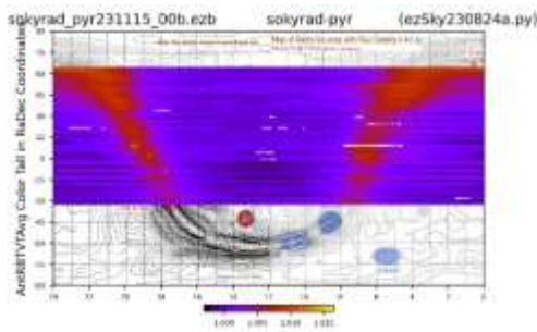
Figure 2: RaDec Plot
