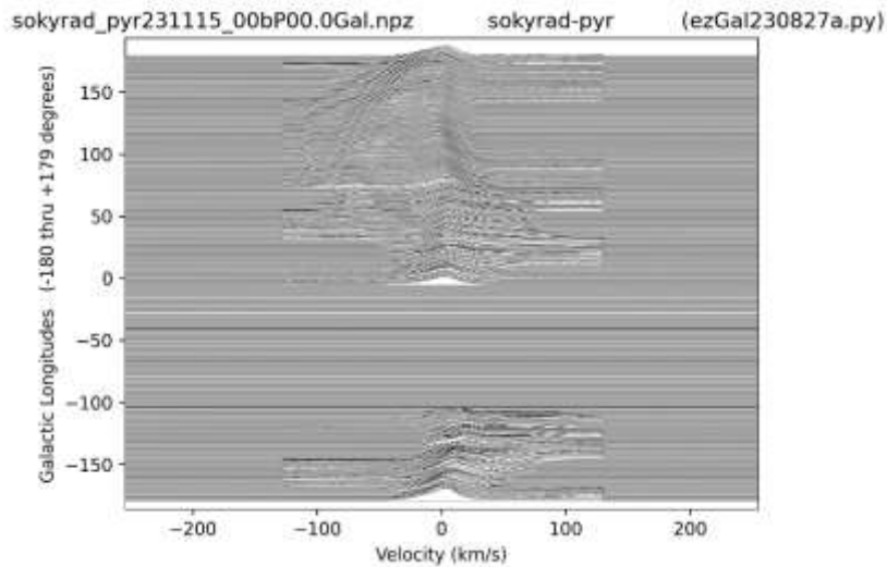
Figure 9: Spectrograph per Galactic Longitude vs. Velocity
