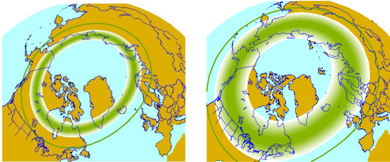
Figure 2 ~ Predictions of the auroral oval and auroral zone in the northern hemisphere. Left : Quiet conditions on 22 September 2023; Right : Comparatively active conditions on 1 December 2023. The wide green belt with white boundaries indicates the predicted auroral oval on the date of the image and the thin green line indicates the approximate boundary for viewing the aurora on the equatorward side of the oval. Note that the poleward boundary of the auroral oval changes very little. Images source: https://www.gi.alaska.edu/monitors/aurora-forecast
