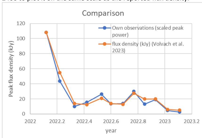
Figure 2: comparison of the measurements from the 1 metre dish with those made by a professional radio observatory
