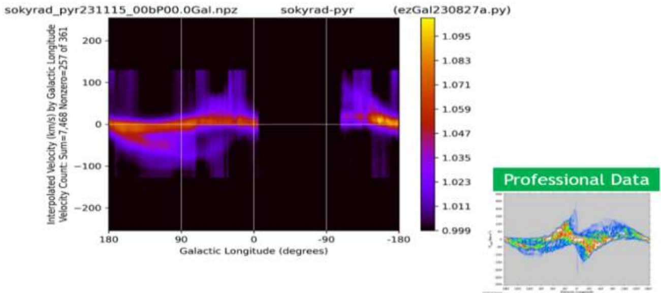
Figure 6: Velocity vs. Gal. Longitude (Professional data [2])
