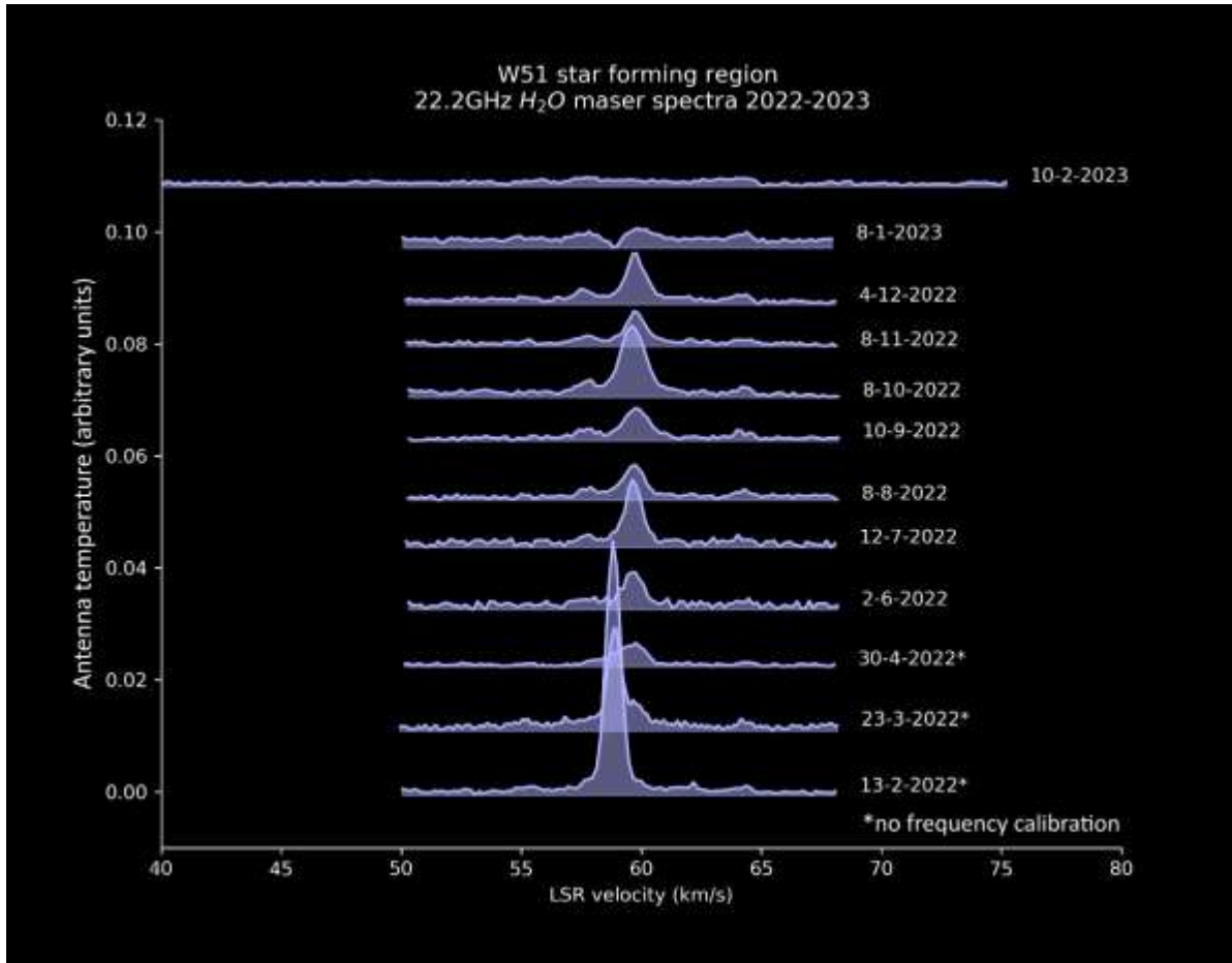
Figure 1: spectra of the 22.2 GHz water maser source in W51. The dates with an asterisk were before the installation of the frequency reference, and the LSR velocities of those spectra therefore have a high uncertainty.:
