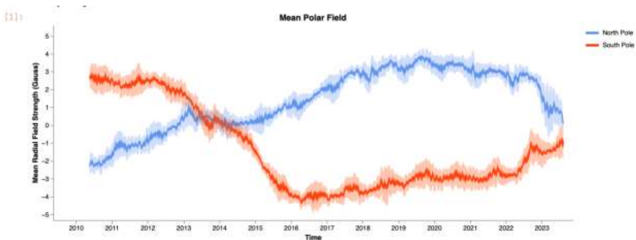
Figure 3 SDO data shows the current solar magnetic field flip beginning in October 2023.
