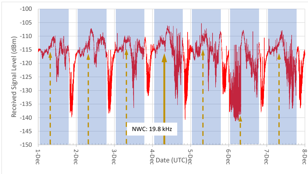
Figure 6.a ~ NWC (19.8 kHz). The daily patterns show approximately 25 dB signal level decrease for a few hours during the local Cohoe morning. The station apparently was off-the-air for several hours on 6 December. A minor signal level dip before peak occurs between around 0100 and 0800 each day, possibly due to sunrise or sunset along the paths.
