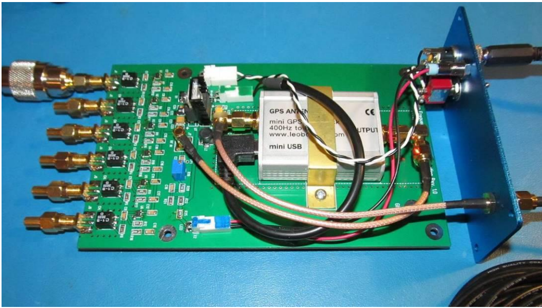
Figure 5 ~ Prototype of the Reference Frequency Distribution System with rear panel while under test. The SMA-F connectors for the six outputs are seen on the left edge of the PCB; channel 1 (upper-left) is connected to the spectrum analyzer for measurements and channels 2 – 6 have 50 ohm terminations. The output transformers are immediately to the right of the RF connectors, and the six identical amplifier circuits are to the right of the transformers. All components are grouped so that the PCB may be cut down and used in a shorter enclosure if the Mini-GPS Reference Clock is not equipped. It is shown here mounted with a metal strap (see text). The power and LED interfaces use friction lock connectors. The prototypes used an MCX-F socket on the PCB (seen here just to the left of the Mini-GPS Reference Clock antenna connection) for connecting the reference source input. This connector was replaced with an SMA-F connector in the production versions. Image ©2020 W. Reeve
