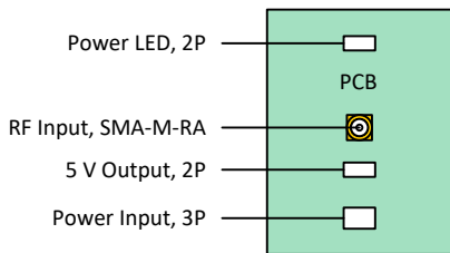
Figure 6 ~ PCB cabling diagram. The RF input uses a threaded RF connector and all other connectors use nylon, polarized, friction-lock wire housings. The connection labeled 5 V Output is for the optional Mini-GPS Reference Clock. The other wire connections go to the rear panel. The RF input connection also goes to the rear panel unless the Mini-GPS Reference Clock is equipped. The power input connector has 3 contact positions to differentiate it from the others; only 2 positions are used. Image ©2020 W. Reeve
