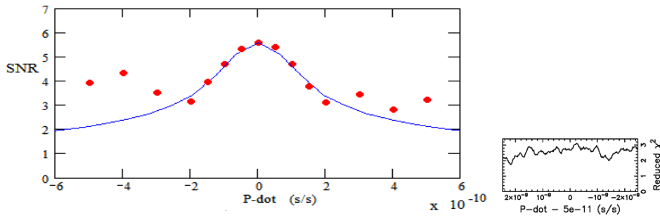
Figure 6. P-dot Search
