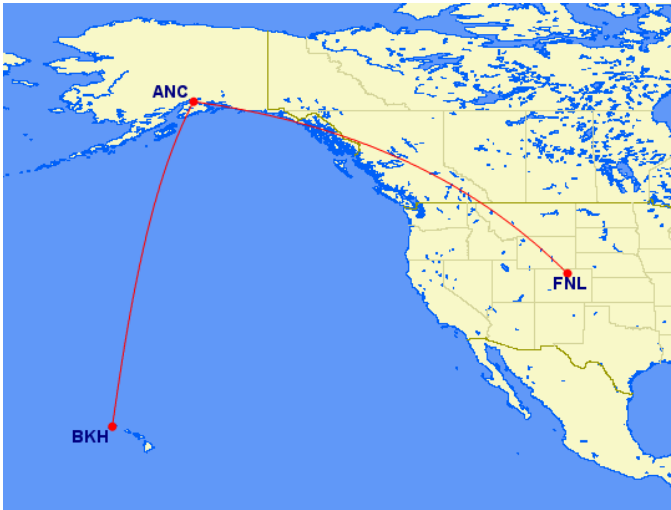
Figure 3 ~ Great circle paths shown in red between WWV near Fort Collins, Colorado (FNL) and Anchorage (ANC) and between WWVH near Kekaha on Kauai, Hawaii (BKH) and Anchorage. The WWVH path is 4414 km and almost entirely over water and encounters different propagation conditions than the WWV path, which is 3801 km and entirely over land. The paths are long enough to require multi-hop propagation. Anchorage is at the southern edge of the auroral oval, which introduces additional complicating factors in propagation toward Anchorage. Image from {GCMaP}.
