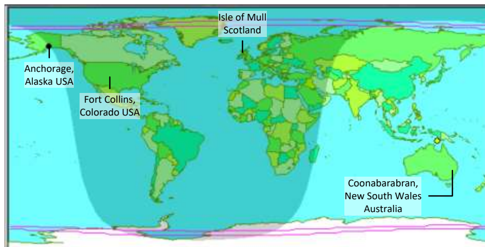
Figure 4 ~ Solar terminator at 0230 UTC on 12 October with marked station locations. The station locations with respect to the Sun were: Anchorage, Alaska USA – On sunset solar terminator; Isle of Mull, Scotland – Near solar midnight; Coonabarabran, New South Wales Australia – Near solar noon (see yellow circle, which represents the Sun); Fort Collins, Colorado USA – about 2 h after local sunset. Underlying image source: {DXViewer}
